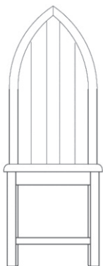
Cathedral Chair H 1185 W 450 D 530
