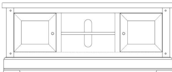
Plasma TV unit H 550 W 1400 D 450
