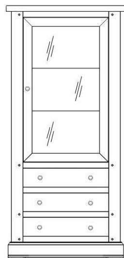
Glazed Display Cabinet H 1750 W 820 D 380
