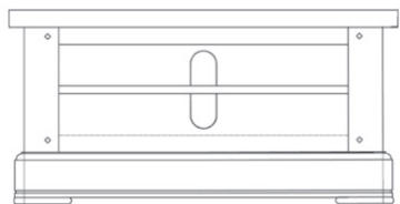
Small TV unit H 450 W 900 D 450
