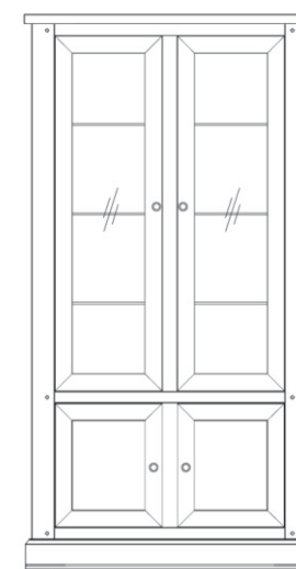
Glazed Cabinet H 1975 W 1040 D 380
