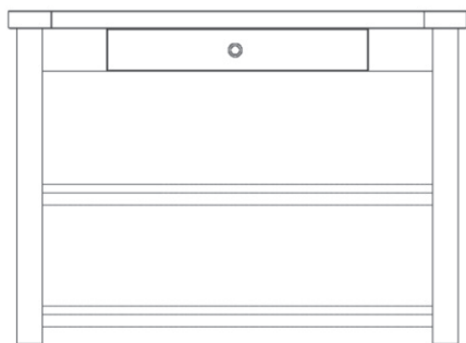
Console table H 790 W 1070 D 350
