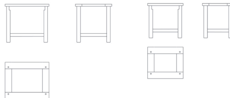
Nest of Tables Large Table H 520 W 600 D 500
