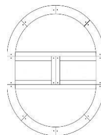
Petite Ox Bow Extended Dining Table w/2 leaves Closed L 1450 x W 900 x H 770 Open (1 inset) L 1800 x W 900 x H 770 Fully open (2 insets) L 2150 x W 900 x H 770
