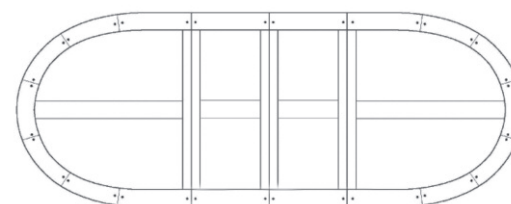
Oval Extended Dining Table w/2 leaves Closed L 1800 x W 1000 x H 790 Open (1 inset) L 2200 x W 1000 x H 790 Fully open (2 insets) L 2600 x W 1000 x H 790
